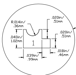
DETAIL OF CASTELLATION PAD 1
