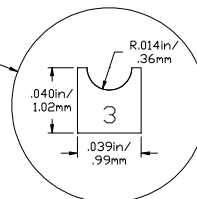
DETAIL OF CASTELLATION PAD 2-6
