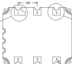
DETAIL OF CASTELLATION PAD 2-6
