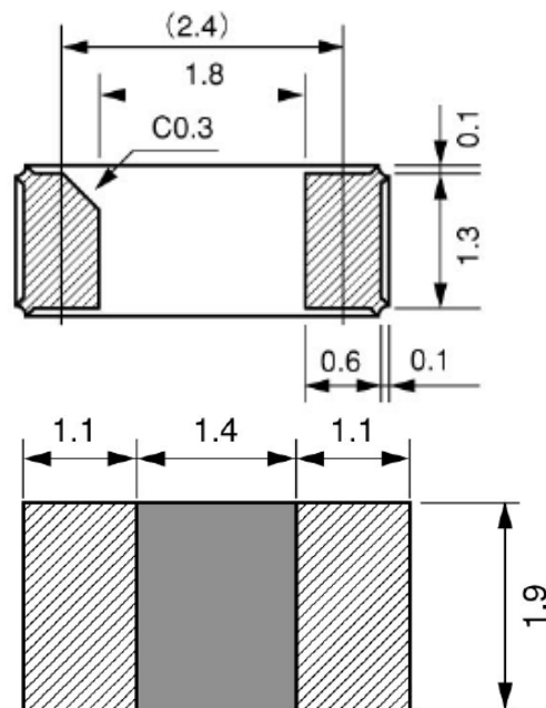
Figure 2) Bottom View and Suggested Land
