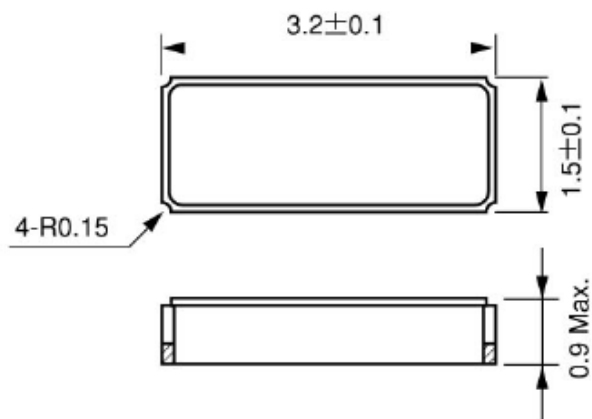
Figure 1) Top and Side View
